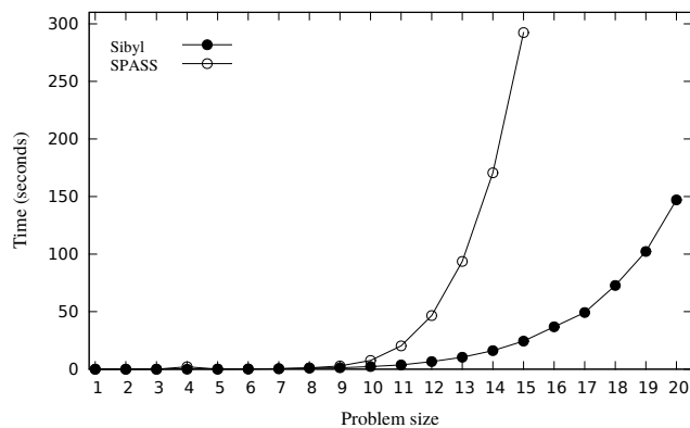
Figure 1: SPASS and Sibyl on the hand-tailored formulae
